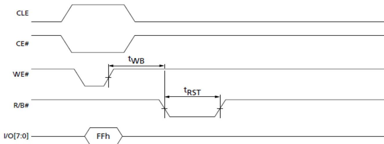
Figure 22 : Reset operation timing
