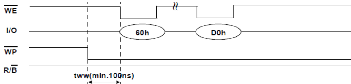
Figure 25 : t_{WW} in Erase Operation
