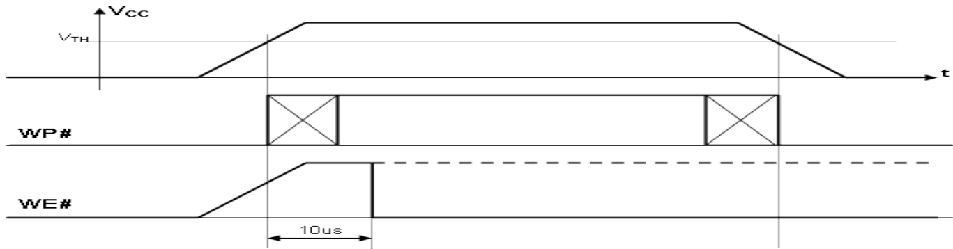
Figure 26 : Power on and Data Protection timings
