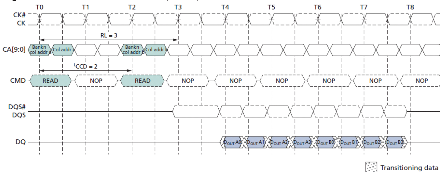
Figure 12: Seamless Burst READ – RL = 3, BL = 4, CCD = 2
